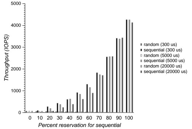
(b) Throughput, with sequential (0, 0) results omitted
