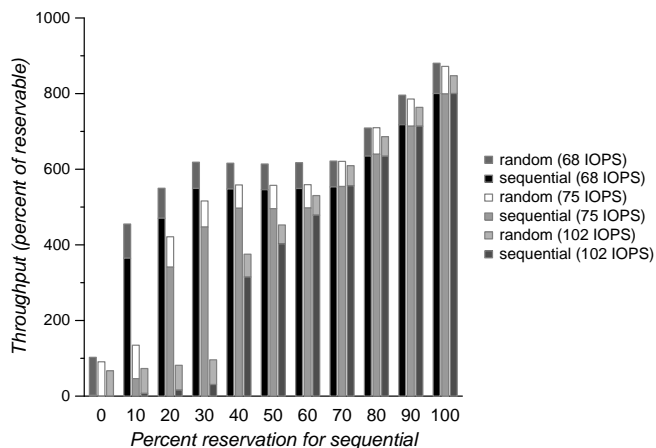
(a) Percent of nominal throughput
